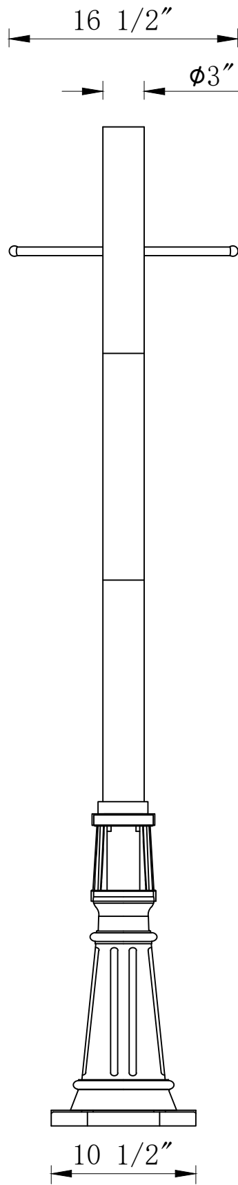
FRONT VIEW
