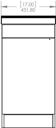
Front view / Vista Frontal
