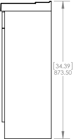
Side View / Vista Lateral
