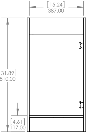
Back View / Vista Trasera
