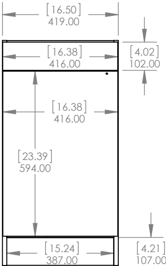
Front view / Vista Frontal
