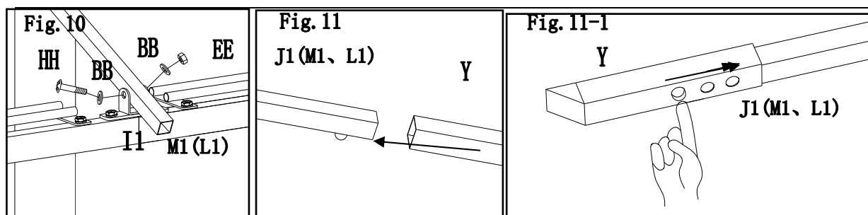
Fig.10: Fix long middle beam(L1) and short middle beam(M1) to middle beam connector(I1), by using bolt (HH)、flat washer (BB) and nut (EE) .
