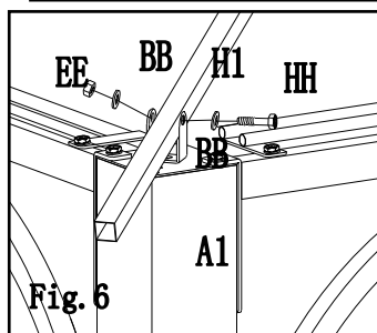
Fig.6: Attach slanting beam bottom tube(H1) to top of post (A1),fix by using bolt (HH)、 flat washer (BB) and nut (EE) .
