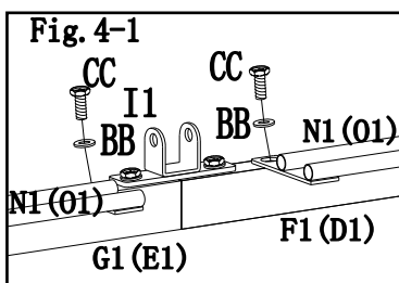
Fig.4-1、 Fig.4-2: Attach netting bar (N1、 O1) to across beam(F1、 D1、 G1、 E1),then fix by using bolt (CC) Flat washer (BB) .
