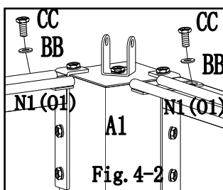
Fig.4-1、 Fig.4-2: Attach netting bar (N1、 O1) to across beam(F1、 D1、 G1、 E1),then fix by using bolt (CC) Flat washer (BB) .
