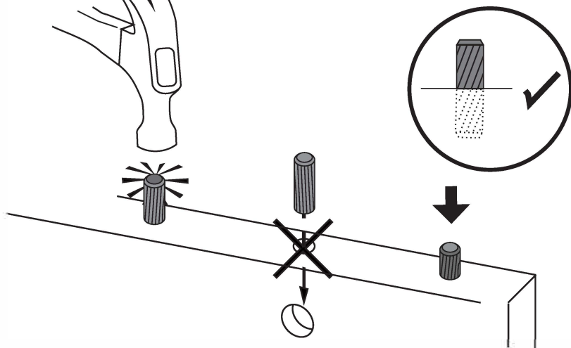
WOODEN DOWELS TARUGOS
