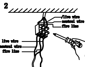
Connect the power cord
