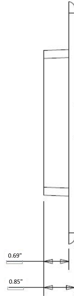
Drywall Frame - Top View
