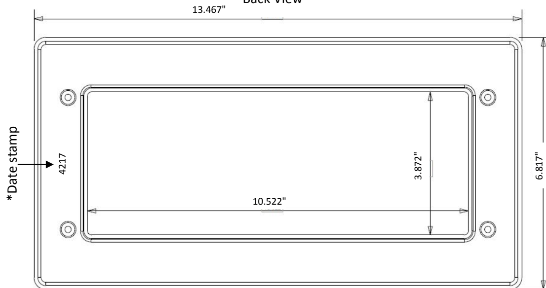
Drywall Frame - Back View
