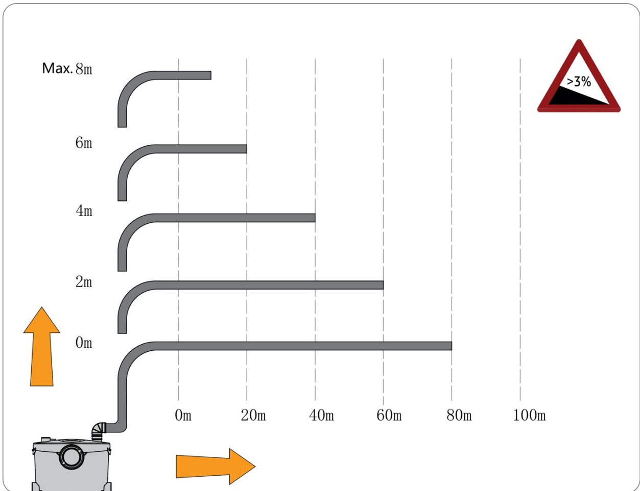
Fig10: Pumping head
