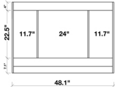
MIRROR VIEW
