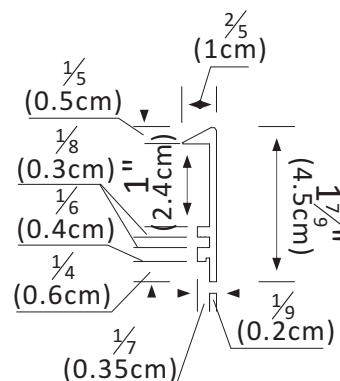
Aluminum section
