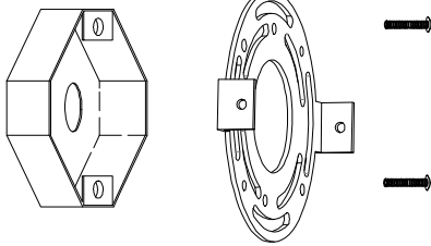
1. Install Metal Bracket to Ceiling
