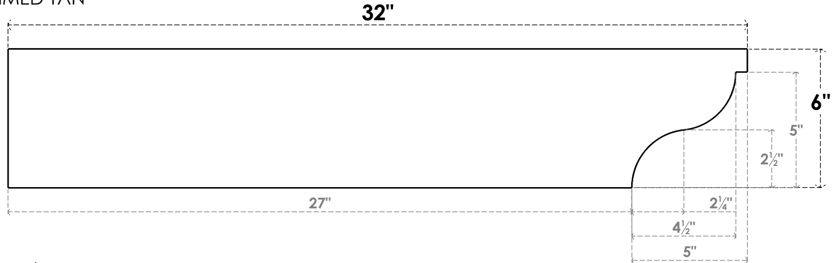
SIDE PROFILE
