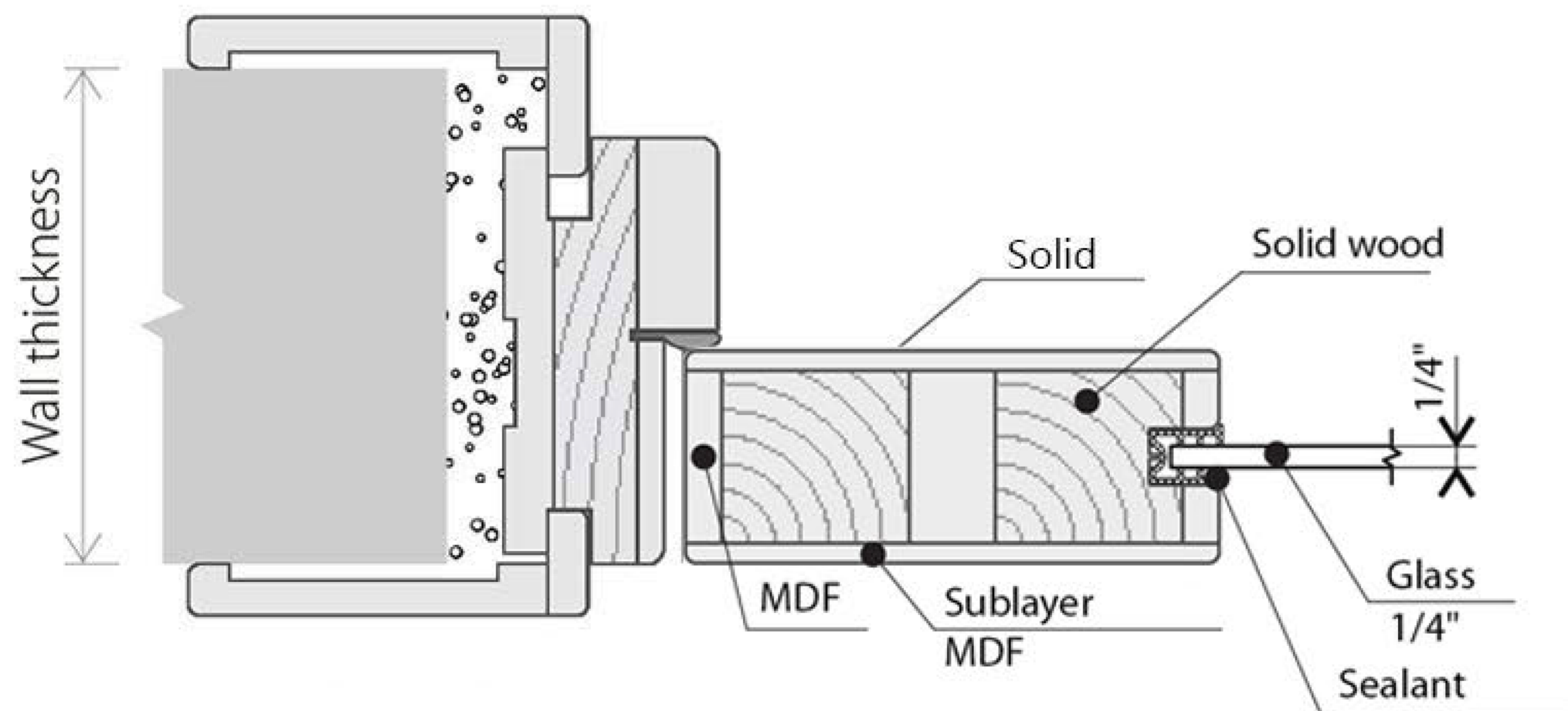
DOOR CUTAWAY VIEW
