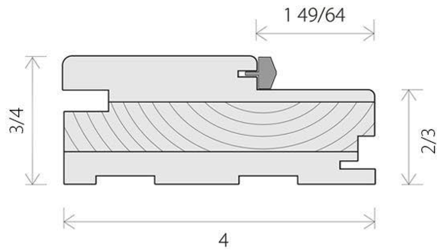
SINGLE JAMB
