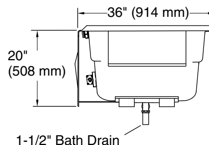
Integral Flange Detail
