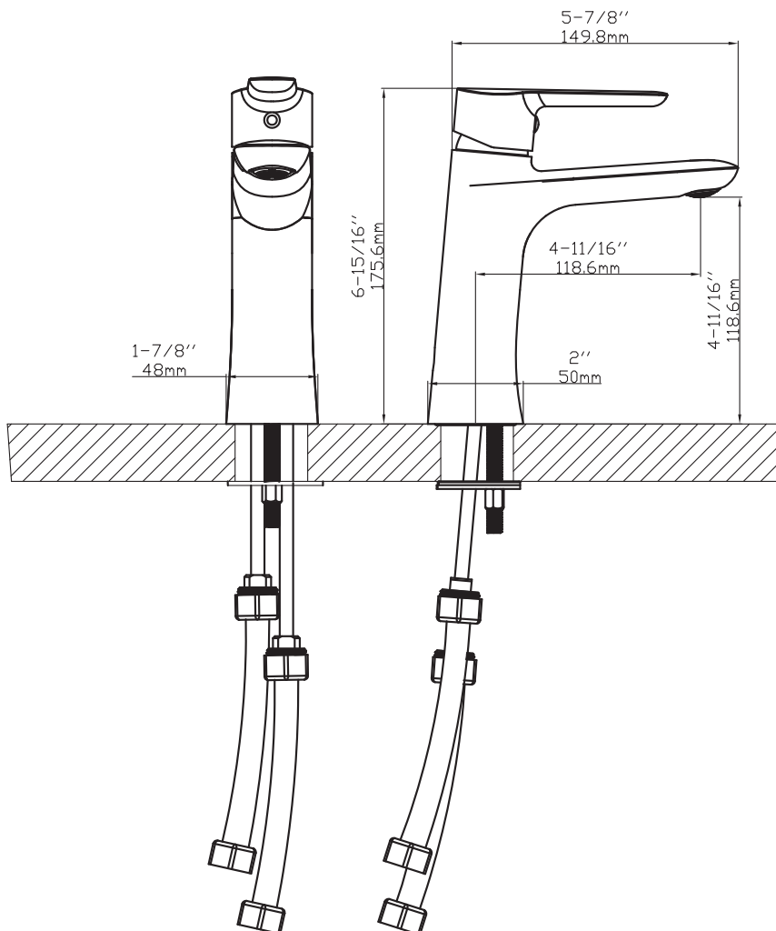
CRITICAL DIMENSIONS
