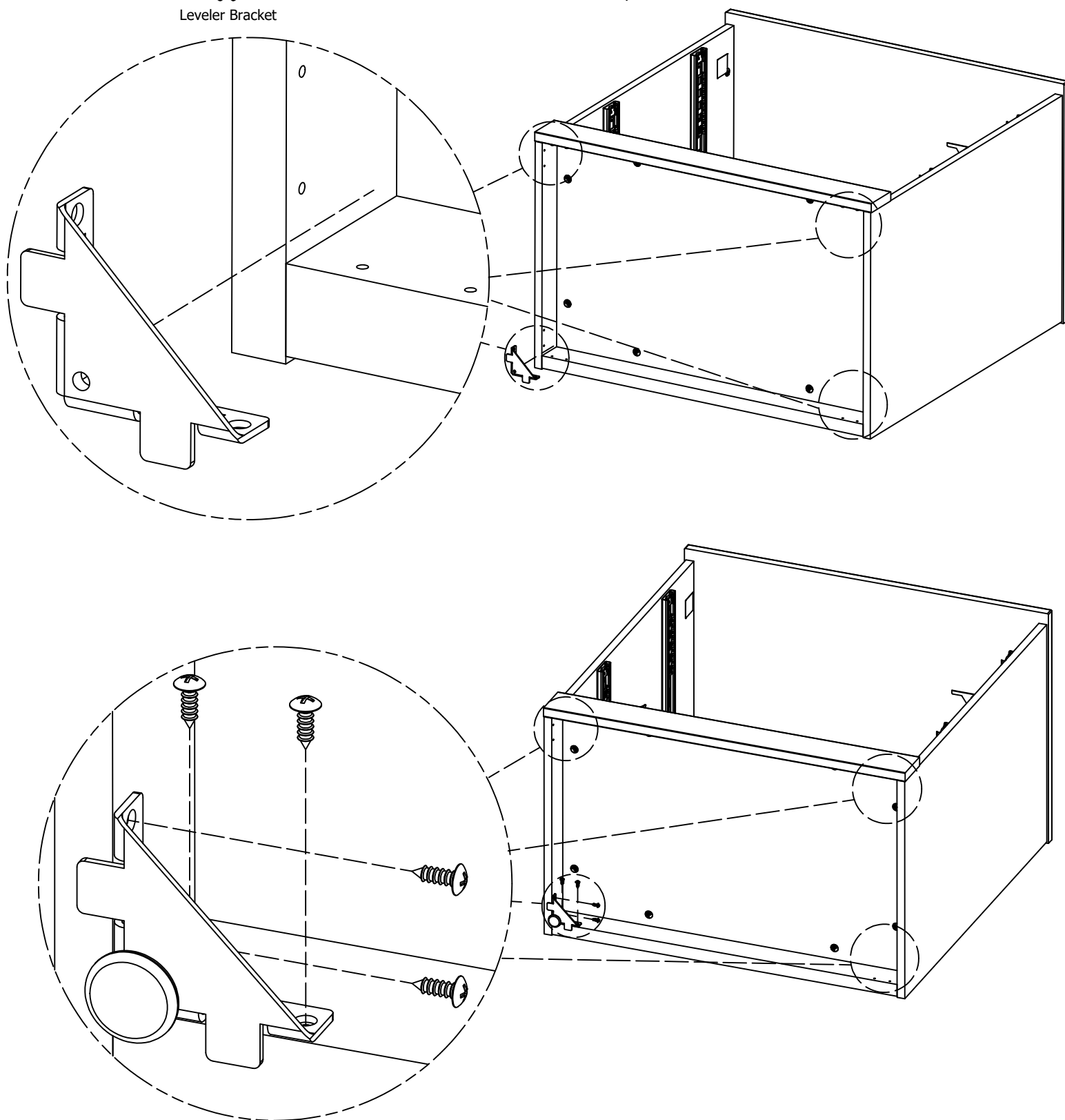
Leveler Bracket
