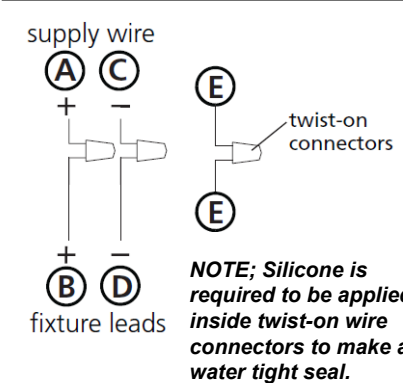
Drawing 3 – Post-Mount
