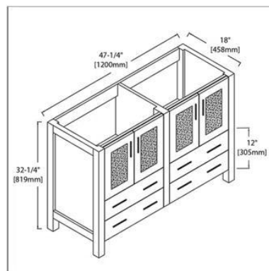
VANITY FRONT
