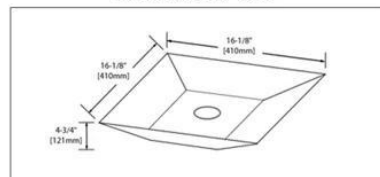
SINK
