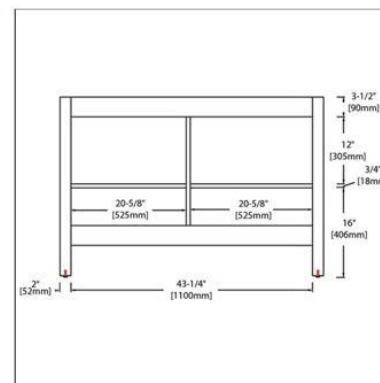
VANITY BACK
