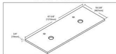
COUNTER-TOP
