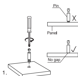
Connecting piece
