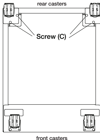
FIGURE 3: Complete assembly.
