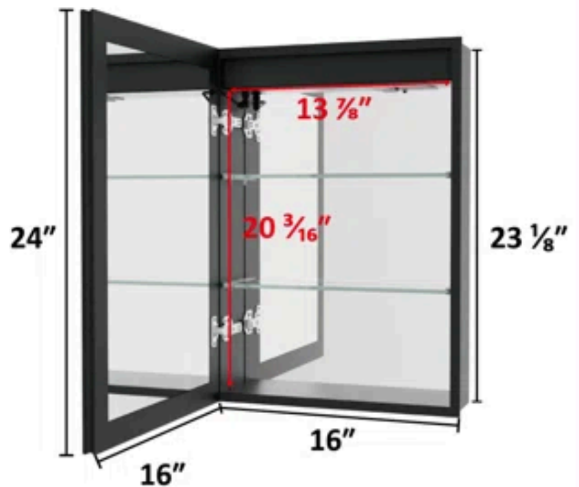
Cabinet Dimensions
