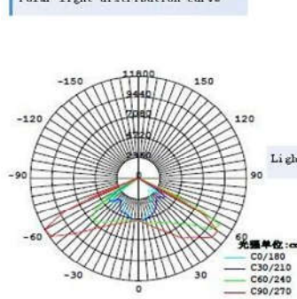
Polar light distribution curve
