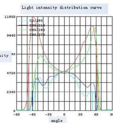
Coordinate light intensity distribution curve
