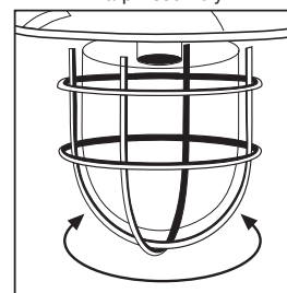
E5 Figure 6 Screw on Glass Assembly
