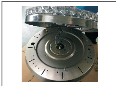
Step 2. Connect the light source driver cable on the lampshade to the power cable on the chassis of the fan lamp host.
