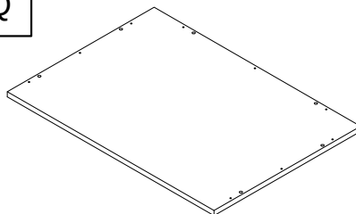
Right Table - Bottom Panel (1PC)
