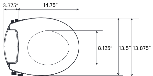
Round Top View
