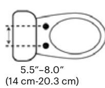
Distance between Bolt Holes
