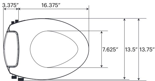
Elongated Top View
