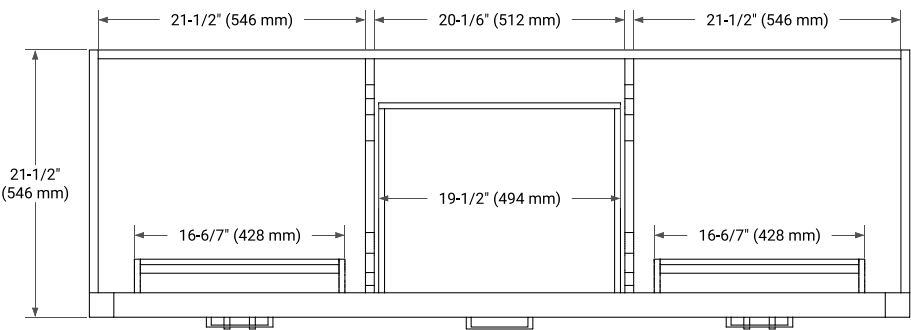
PLAN VIEW
