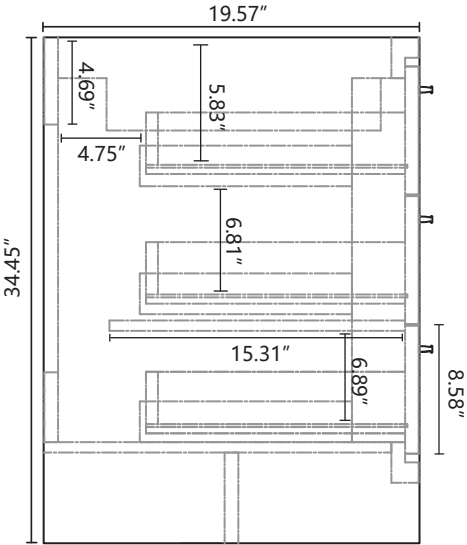
Side Elevation
