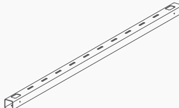
Horizontal Top Rail (2) 1 1/2" x 1 1/2" x 44"
