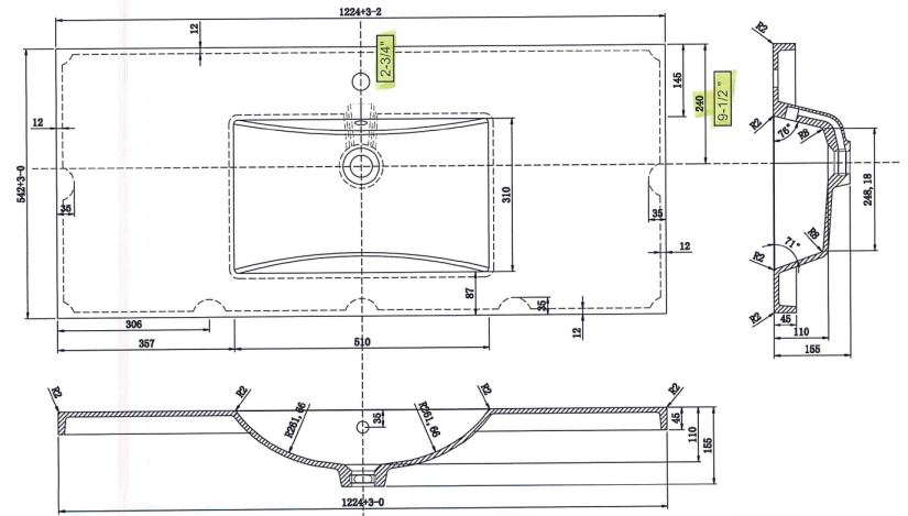
SINK DETAIL
