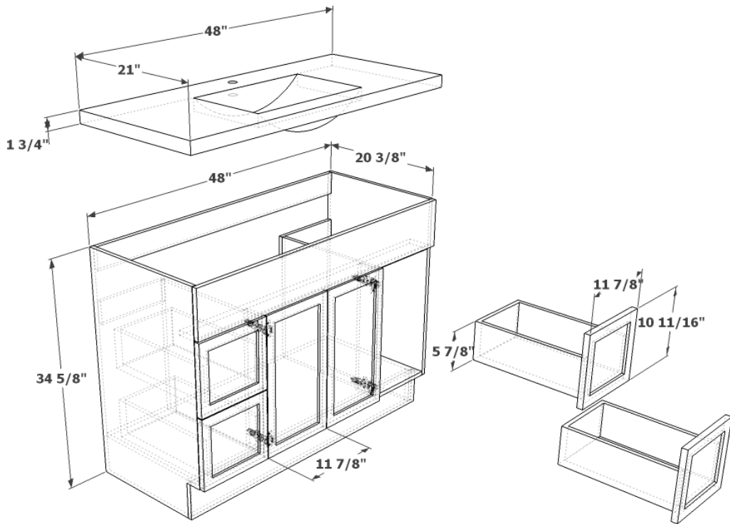
SINK DETAIL
