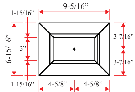
— SMALL DRAWER —
