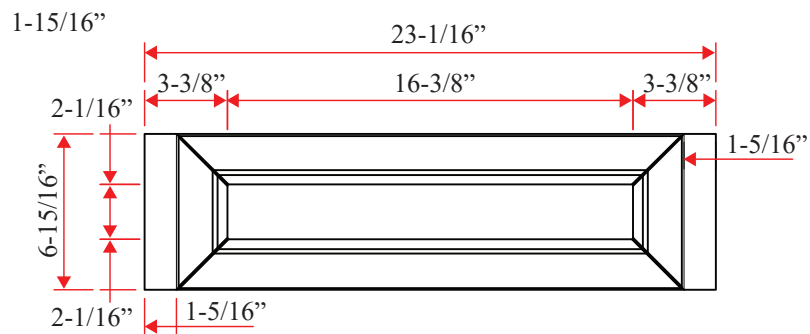
— FAKE DRAWER —
