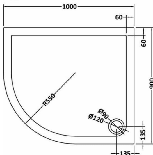
1000 x 900 OFFSET QUADRANT TRAY LH
