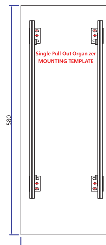
Drilling Template
