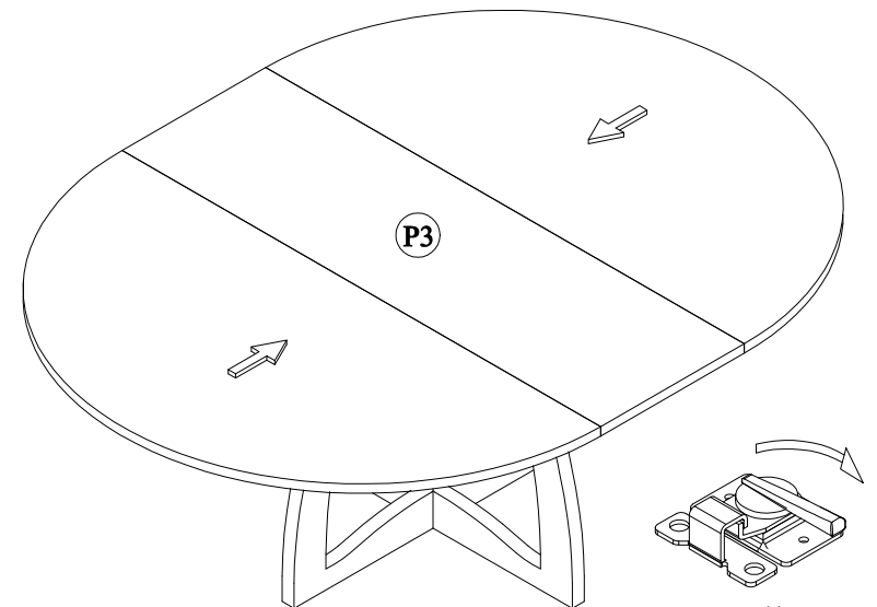
Detail 'C'
