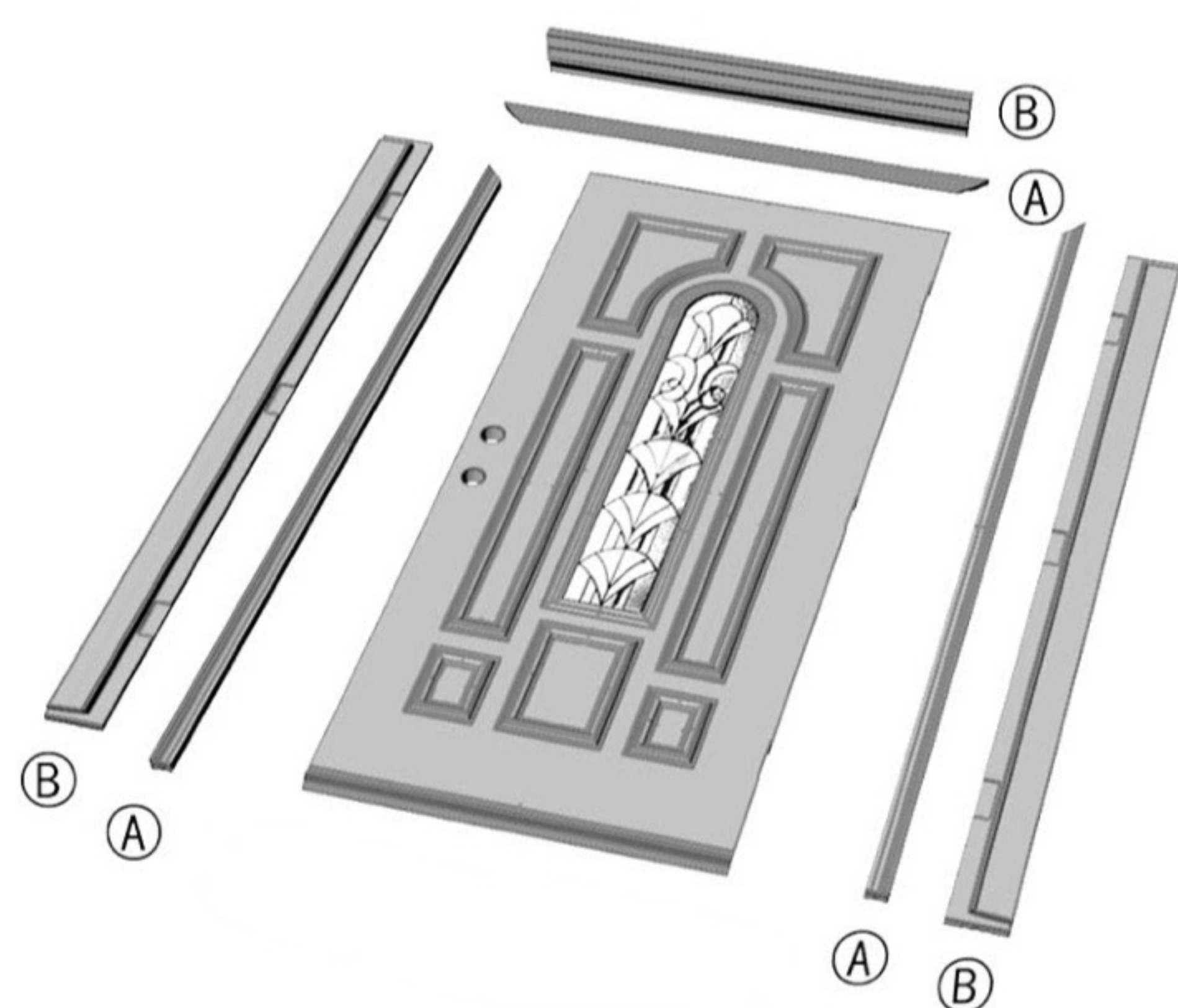
BASIC PARTS&COMPONENTS
