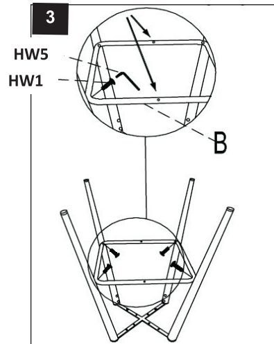
Step 3 Then put the footrest(B) in the middle of Iron legs as picture showed And used the Allen keyM5(HW5) to fix with Flat Hex bolts(HW1).
