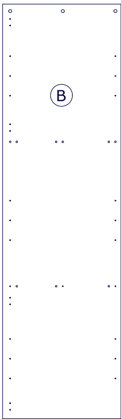
● TR1636 2015x576x16mm
