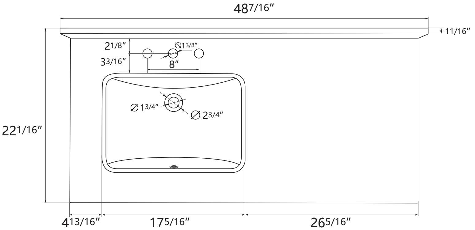
Top View
