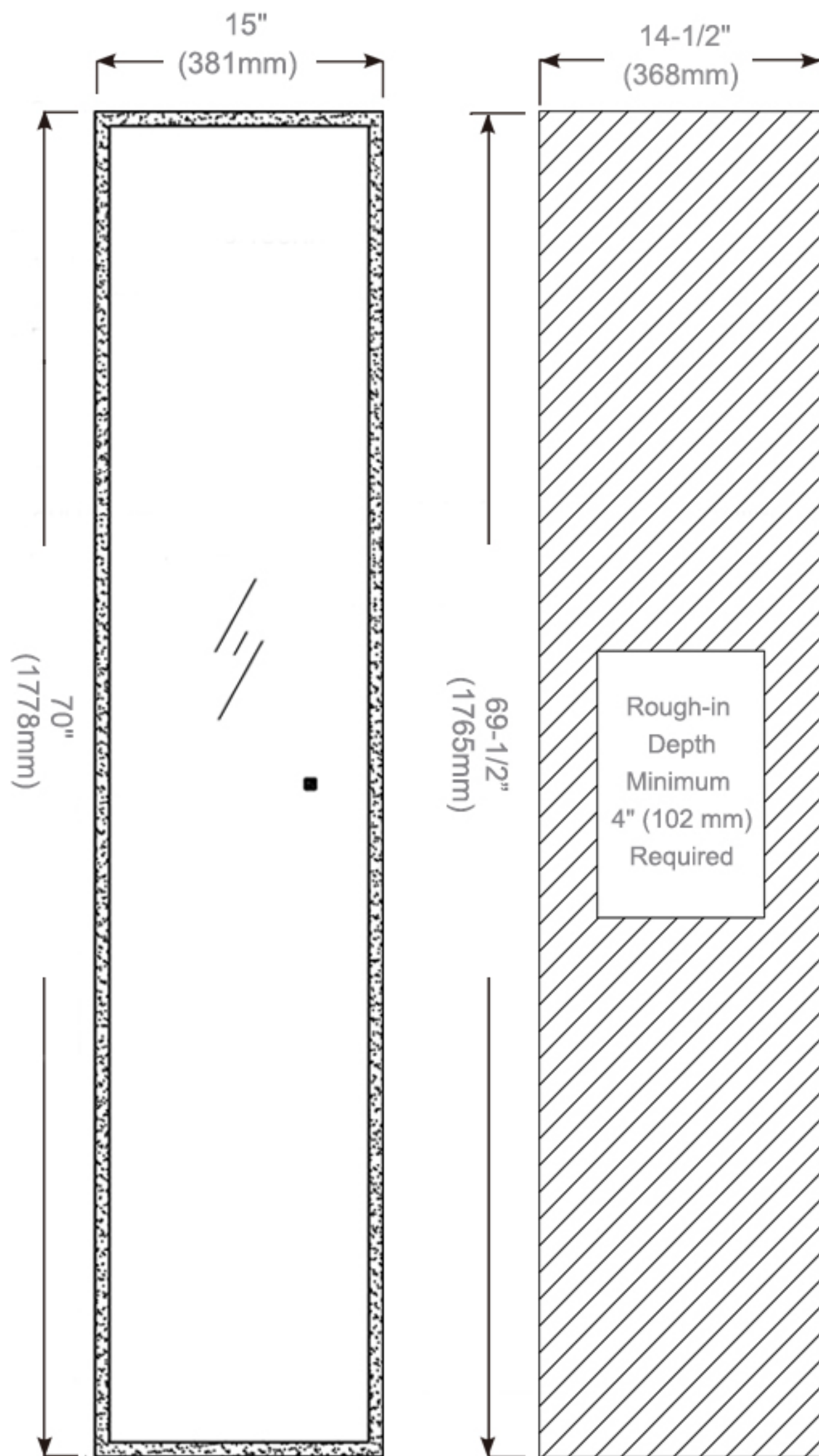
Cabinet Dimensions
