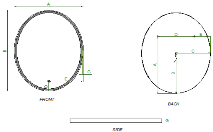
FRONT & SIDE
