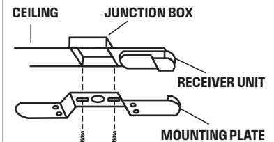
FIGURE - 5 FLUSHMOUNT FANS ONLY
