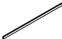
Horizontal bar 1992x60x25 mm 1 pc Barre horizontale 1992x60x25 mm
