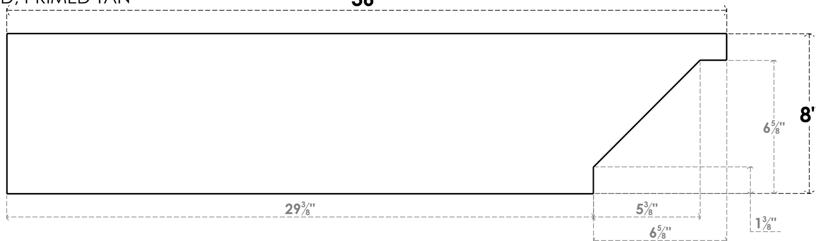
SIDE PROFILE
