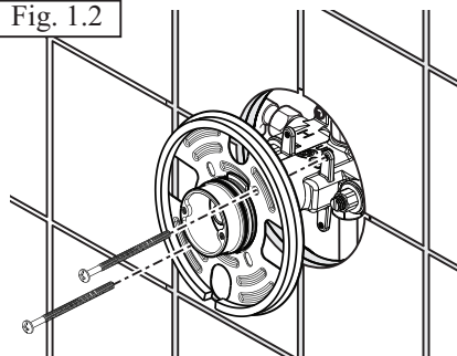
Valve 1/2" 101559
