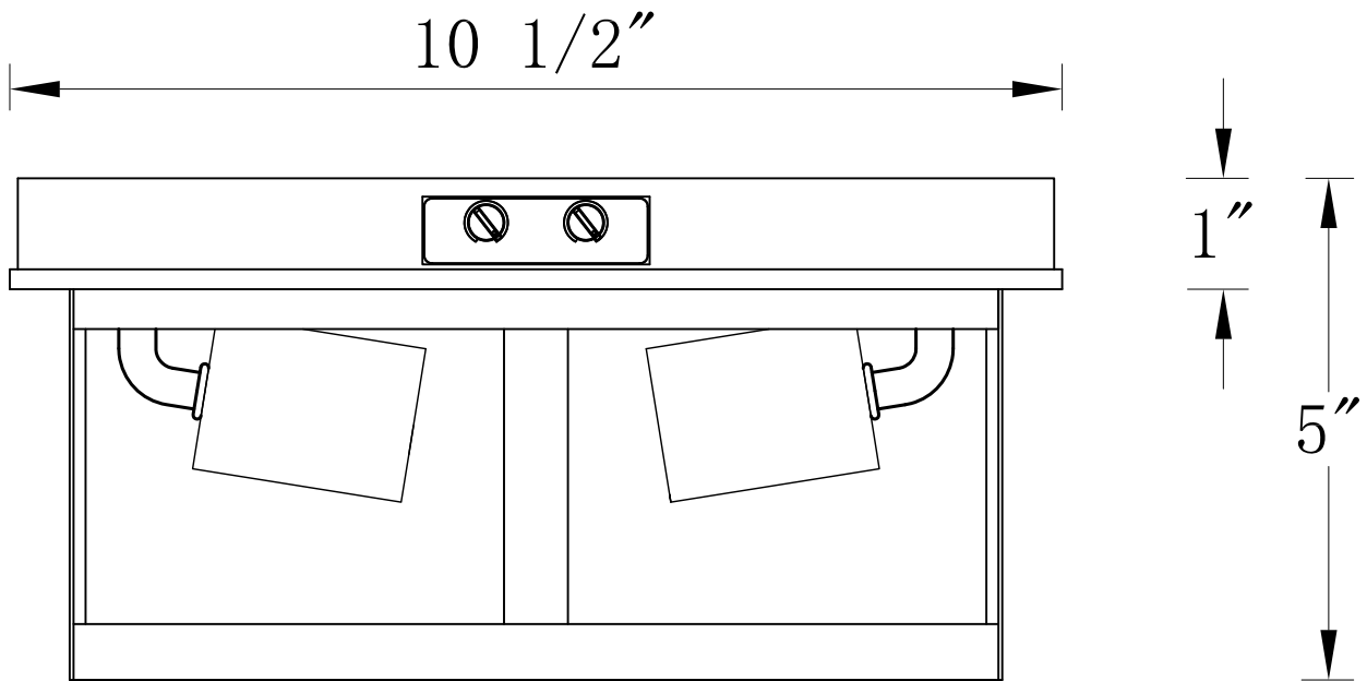
FRONT VIEW
