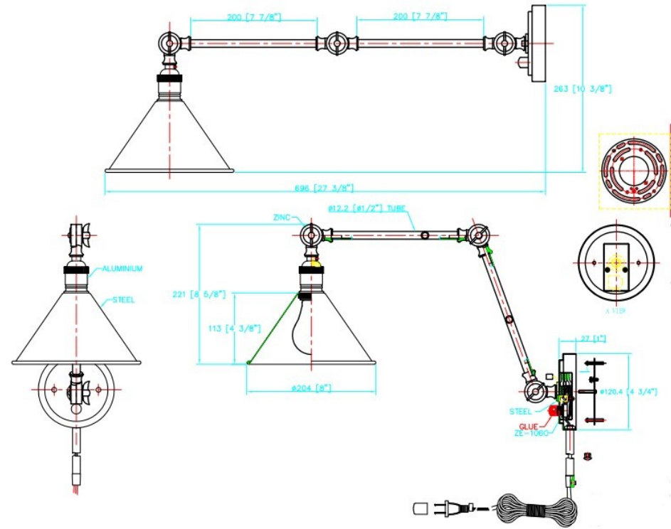
Portable Fixture
