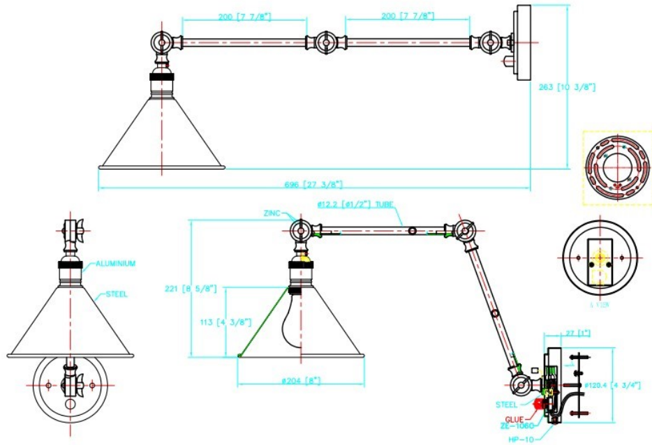
Hardwired Fixture
