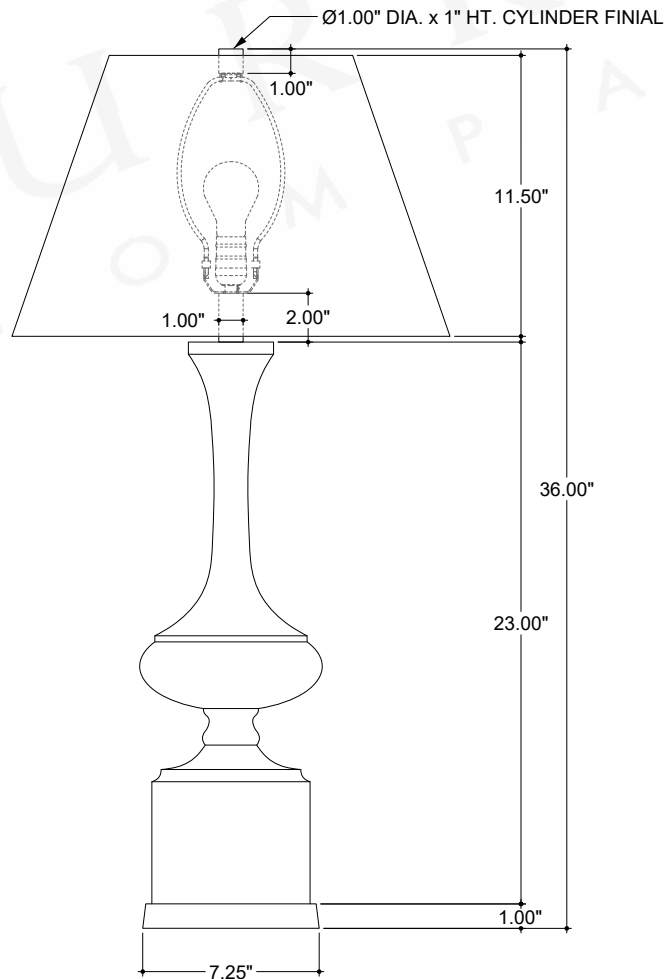
FRONT VIEW
