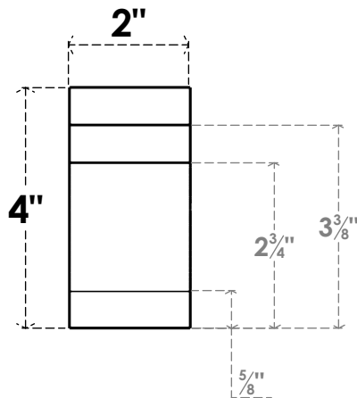
FRONT PROFILE
