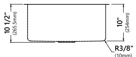
KHU121-23 23" x 18 3/4" x 10" Min Cabinet Size: 27" Matching Grid: KBG-121-23 Drain Model #: BST-1
