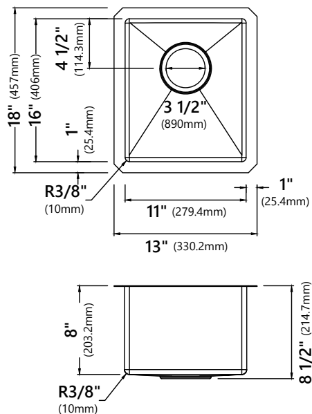
KHU101-13 13" x 18" x 8" Min Cabinet Size: 15" Drain Cap #: STC-2 Drain Model #: ST-1
