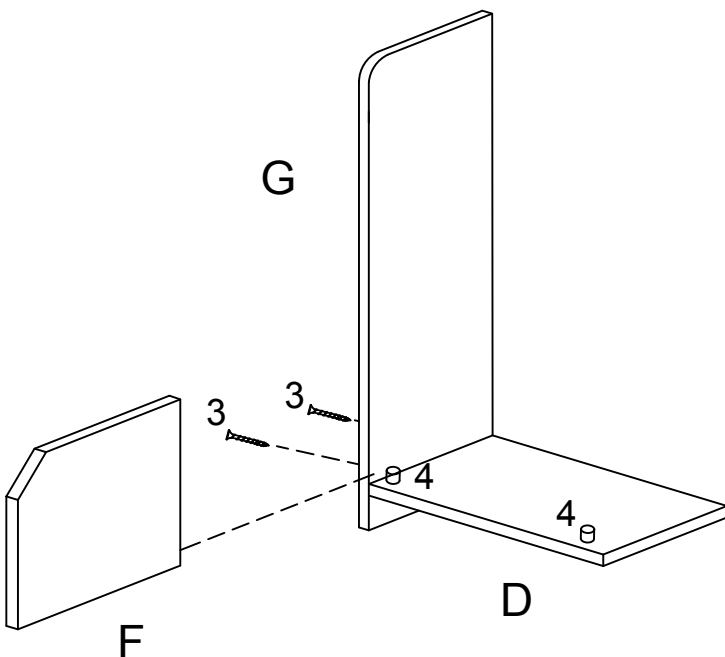
Install panel through fitting 3 and 4.
