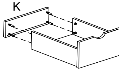
Install drawer back plates.
