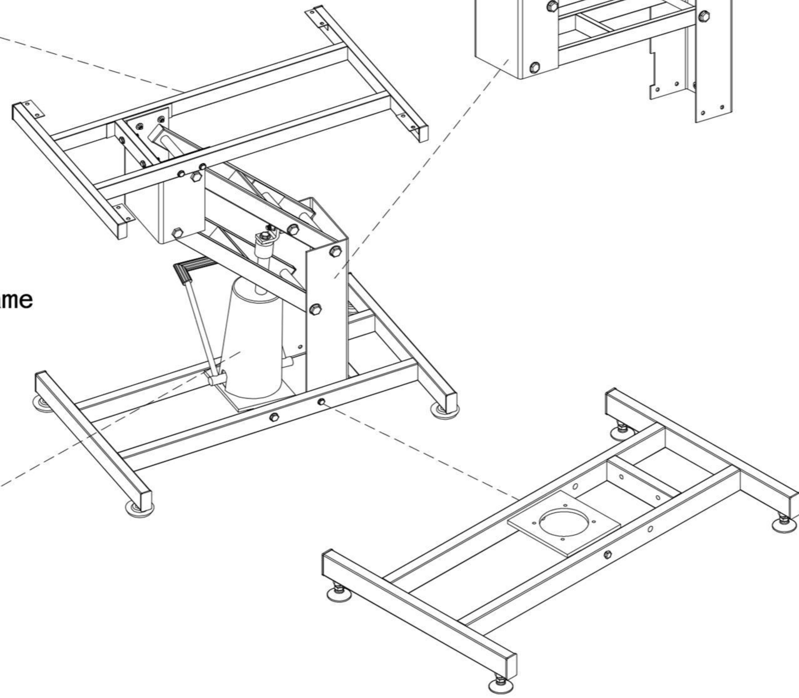
① Frame equilibrium frame
